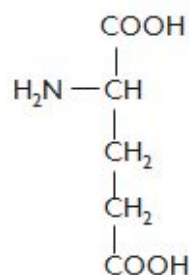
glutamic acid
