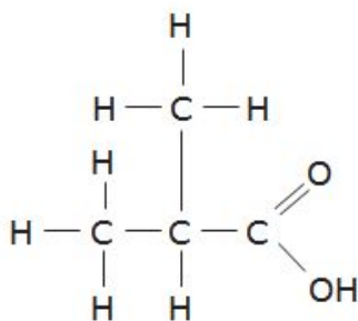
2-methylpropanoic acid
