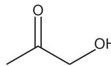
Acetol
