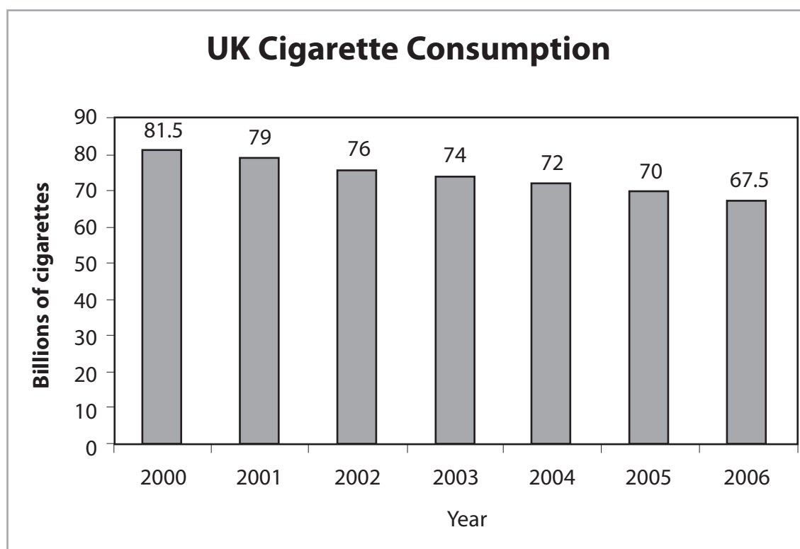
Figure 1: UK Cigarette Consumption (2000 – 2006)
