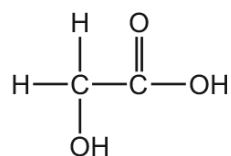
glycolic acid
