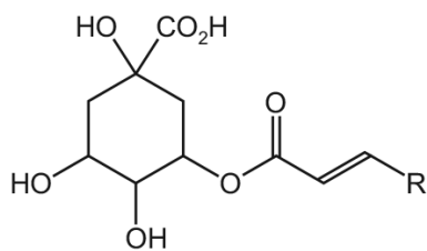
chlorogenic acid
