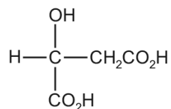
malic acid
