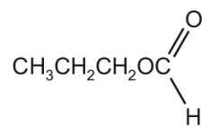
compound X
