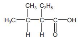
2-ethyl-3-methylbutanoic acid
