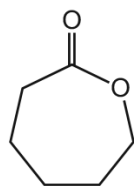
caprolactone
