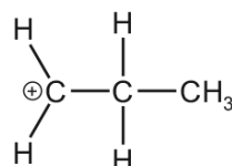
intermediate II
