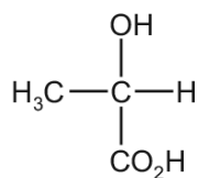
lactic acid
