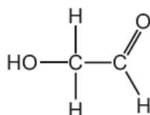
hydroxyethanal
