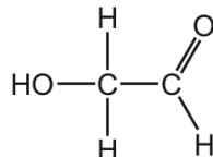
hydroxyethanal
