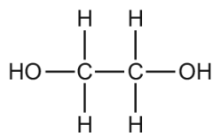
ethane-1,2-diol
