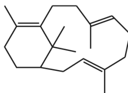
compound Y
