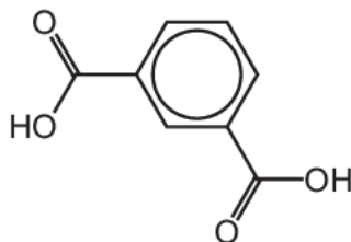
benzene-1,3-dicarboxylic acid
