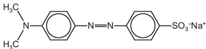
methyl orange
