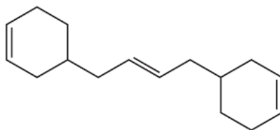
molecule X
