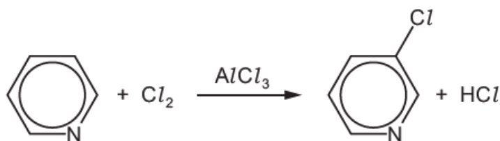
pyridine
