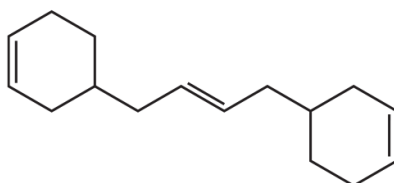
molecule X
