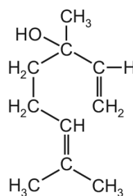
linalool
