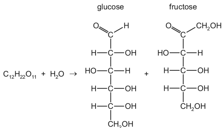
reaction Z
