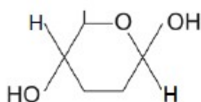
Molecule A
